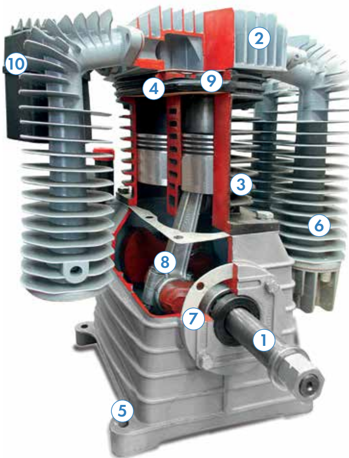
CILINDERS
